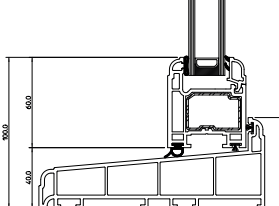
Sideways View - Standard Bottom Rail
